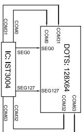
LCD LAYOUT
